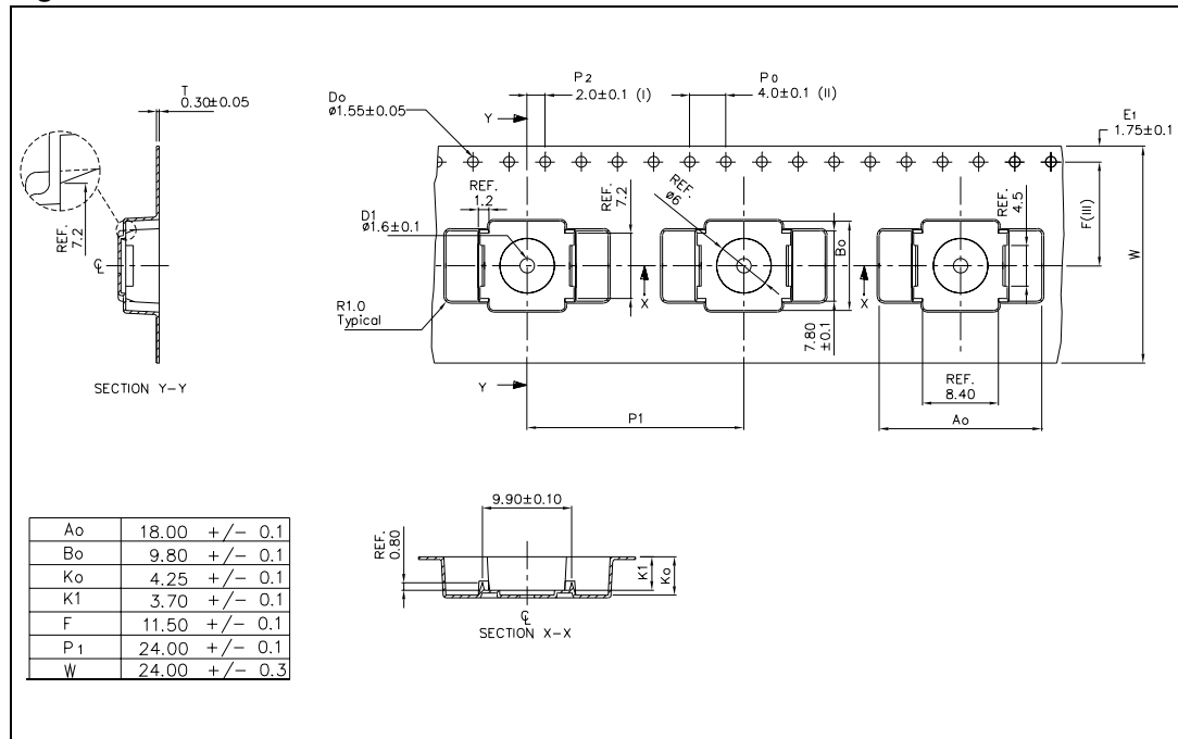
Figure 36. Reel information
